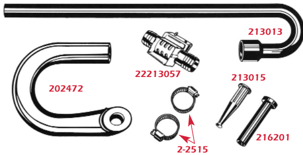
2-4660K MAYTAG INJECTOR KIT Side Mount injection fill assembly for older models
