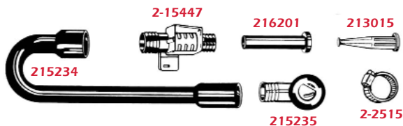
206680 MAYTAG INJECTOR KIT Bottom Mount injection fill assembly for later models
